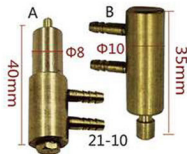
21-10 常闭挂架阀 Normal Close Hanging Valve
